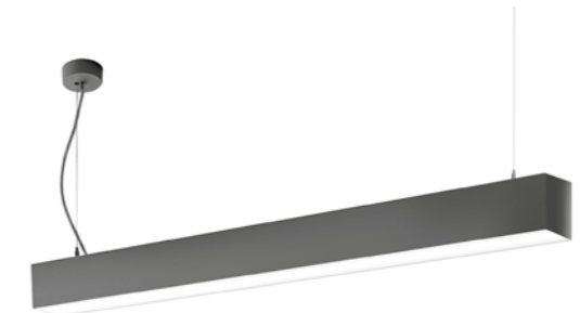
LINE 26/43W - 2400/4000Lm
