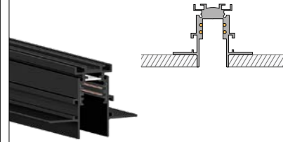
BINARIO AD INCASSO RECESSED TRACK
