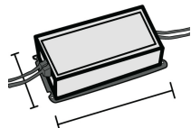
644758 DRIVER Driver ON-OFF 8W 350mA IP20
